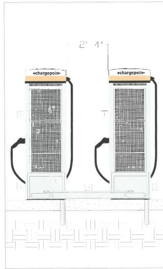
ELEVATION - PAIRED STATION - BACK
