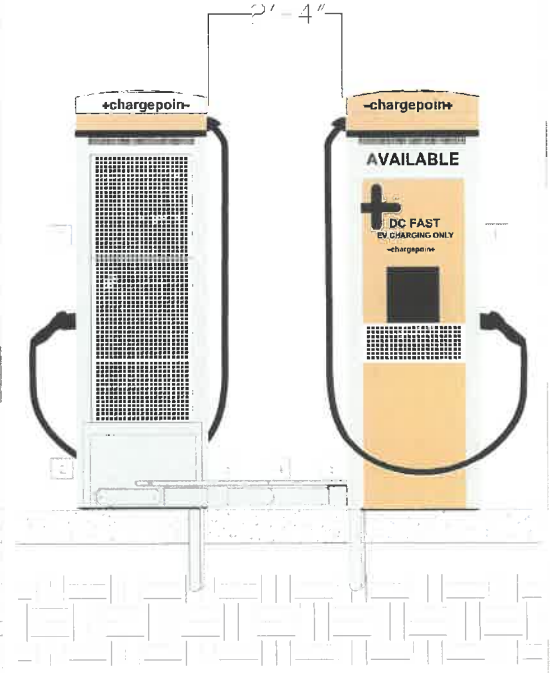
ELEVATION - PAIRED STATION - SIDE
